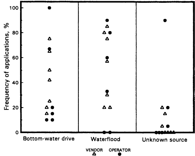
Fig. 6. Distribution of production-well applications.
