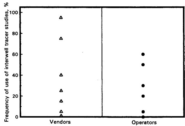
Fig. 10. Frequency of use of interwell tracer studies for diagnosing channeling in waterfloods.
