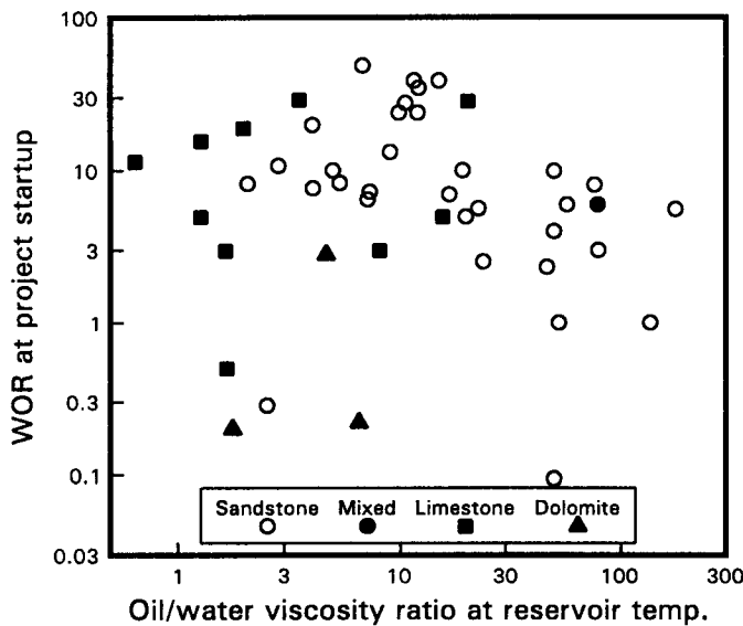
Fig. 1. WOR versus oil/water viscosity ratio for injection-well gel projects.
