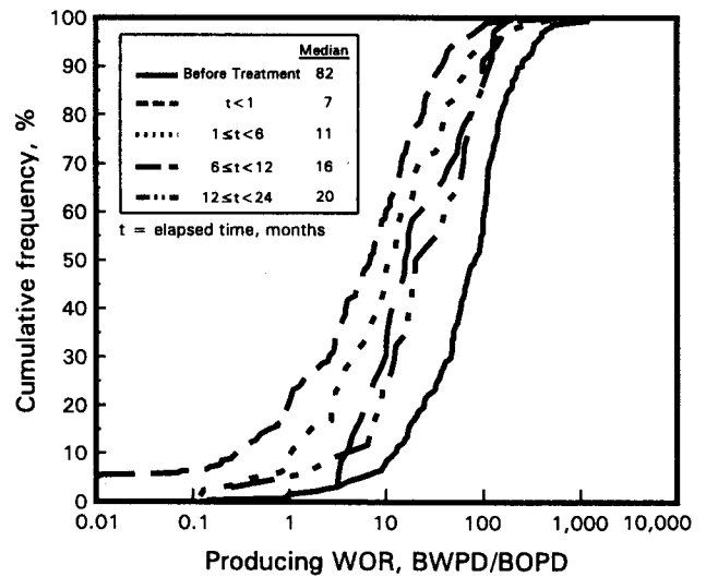
Fig. 4. Cumulative frequency plot of WOR before and after production-well treatments.
