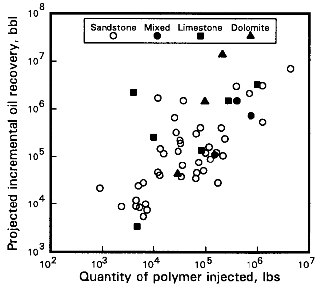
Fig. 2. Projected IOR versus lbs of polymer for injection-well gel projects.
