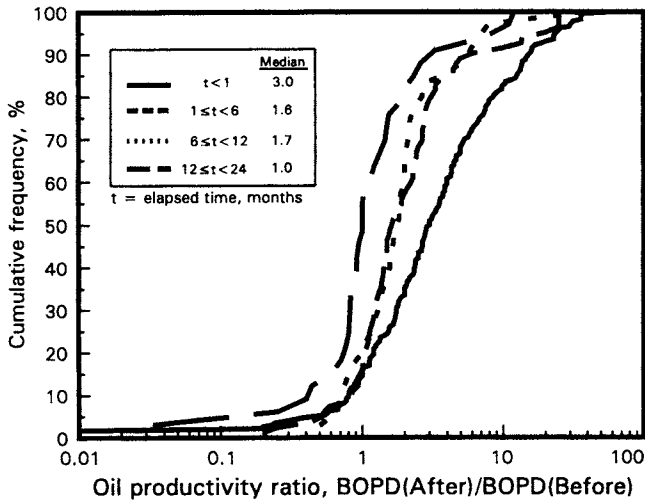
Fig. 5. Cumulative frequency plot of oil productivity ratios before and after production-well treatments.
