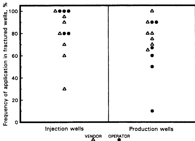
Fig. 9. Frequency of application in fractured wells.
