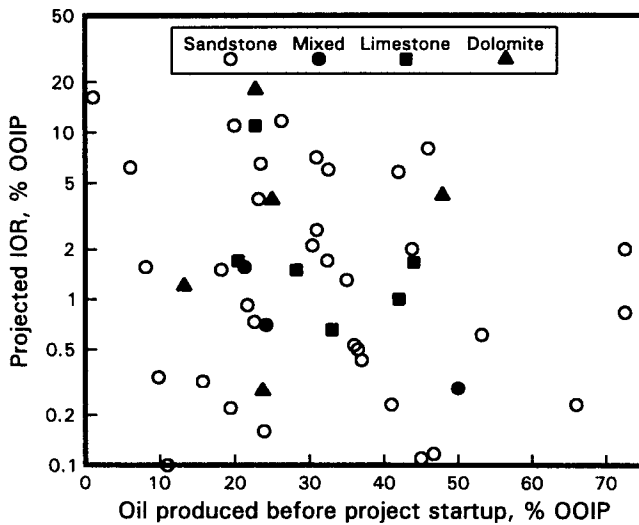
Fig. 3. Projected IOR versus % OOIP produced before startup for injection-well gel projects.
